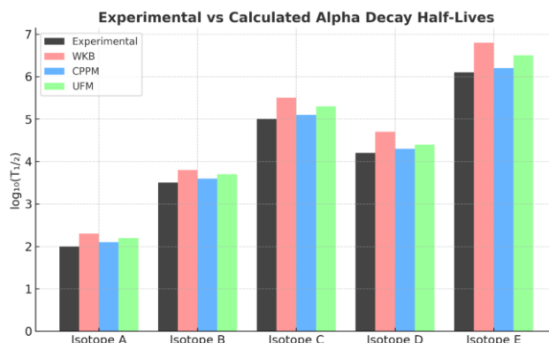
Fig.2. Comparison between experimental and calculated \log_{10}(T_{1/2}) values for selected heavy isotopes using WKB, CPPM, and UFM models.
