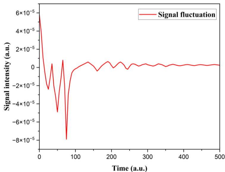
Fig. 5. Temporal evolution of the selected AES signal intensity associated with the Pt(110) surface after the cleaning procedure, showing the transition from the initial transient regime to a stable quasi-stationary state.
