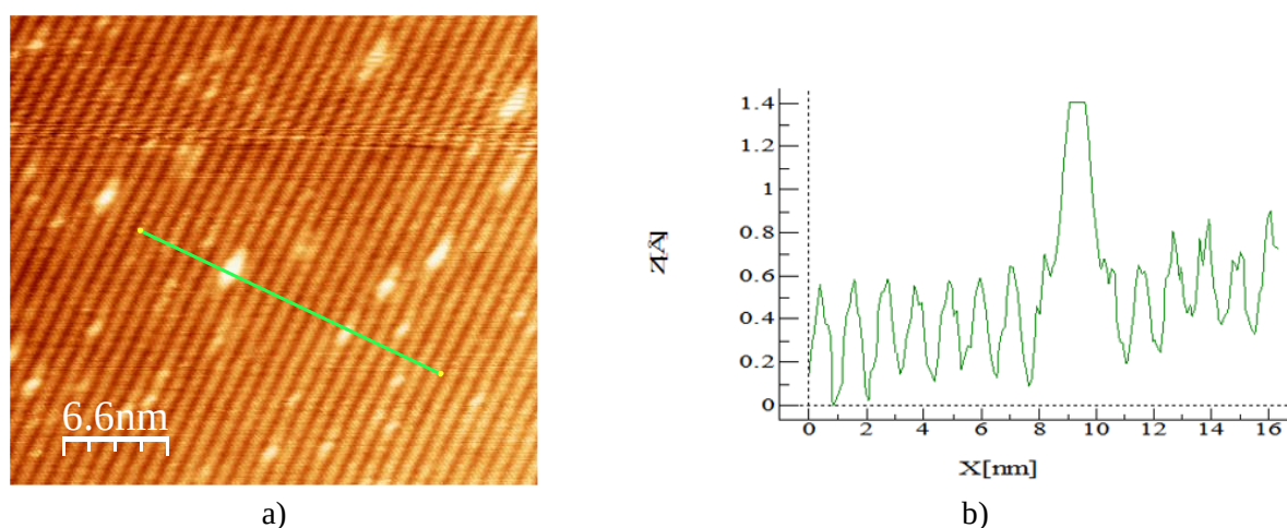
Fig.9. Large-scale STM image of the Pt(110) surface: (a) 33 nm × 29 nm topography; (b) cross-section along the line in (a), indicating the corrugation normal to the [110] rows.
