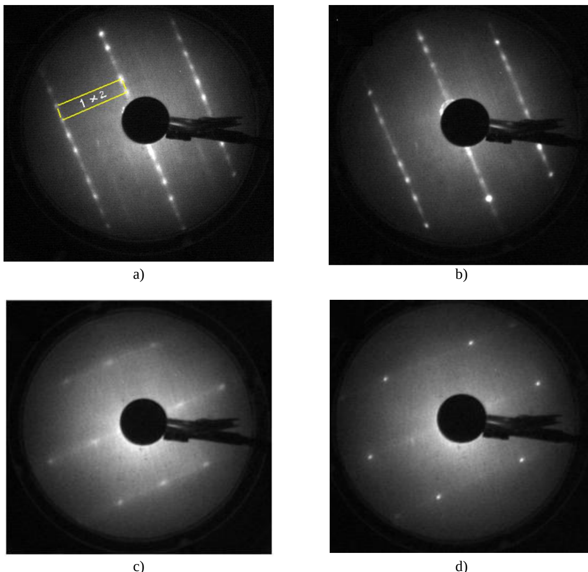
Fig. 6. LEED patterns obtained from the Pt(110) surface and Fe/Pt(110) system at different electron energies after annealing and flashing: (a) clean Pt(110), E_0 = 76 eV; (b) clean Pt(110), E_0 = 84 eV; (c) Fe/Pt(110), E_0 = 82 eV; and (d) Fe/Pt(110), E_0 = 92 eV. Fe deposition partially suppresses the missing-row reconstruction, while the hexagonal pattern in (d) indicates the formation of an ordered Fe overlayer.
