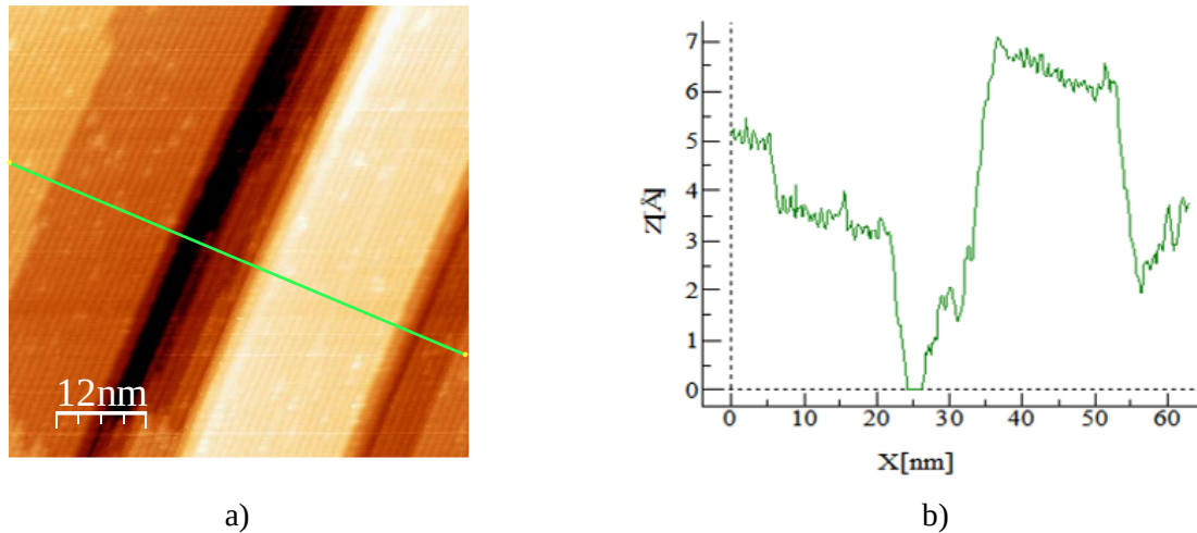
Fig. 7. STM image of the reconstructed Pt(110) surface: (a) topography showing long-range order with step features and (b) line profile along the green line in (a), showing the terrace-step height variation. The well-structured surface confirms the effectiveness of the cleaning-annealing process.
