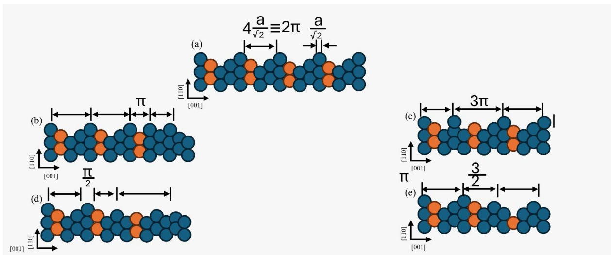
Fig. 2. Side view of the (1 \times 2) reconstructed fcc(110) surface: (a) ideal surface with 4d periodicity along [001] ; (b, c) antiphase domain walls with phase shifts of \pi and 3\pi ; (d, e) surface steps with phase shifts of \pi/2 and 3\pi/2 .
