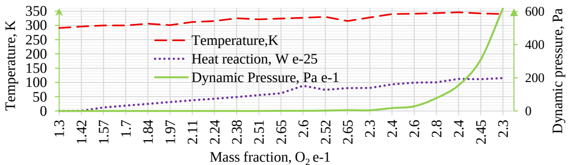
Fig.3. \text{O}_2 mass fraction and heat of oxygen reaction with coal during the diffusion drying process: a – \text{O}_2 mass fraction; b – heat of oxygen reaction with coal.
