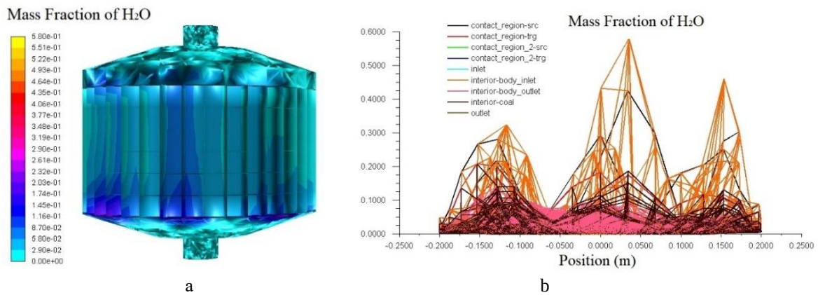
Fig.5. Mass fraction of H 2 O release during the diffusion drying process: a – in common; b – on the perimeter of the chamber.
