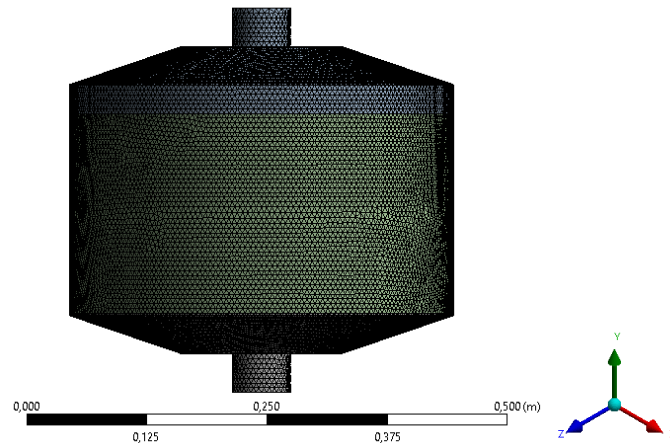
Fig.2. Dynamic mesh selection for drying chamber
