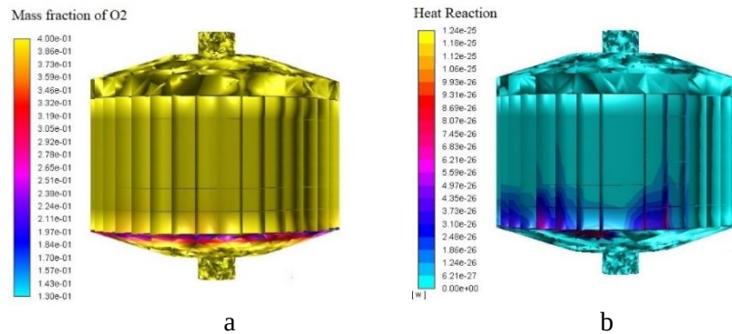
Fig.3. \text{O}_2 mass fraction and heat of oxygen reaction with coal during the diffusion drying process: a – \text{O}_2 mass fraction; b – heat of oxygen reaction with coal.
