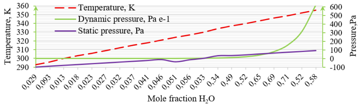
Fig.6. Dependence H 2 O mole fraction from dynamic pressure and absolute temperature during the diffusion drying process.
