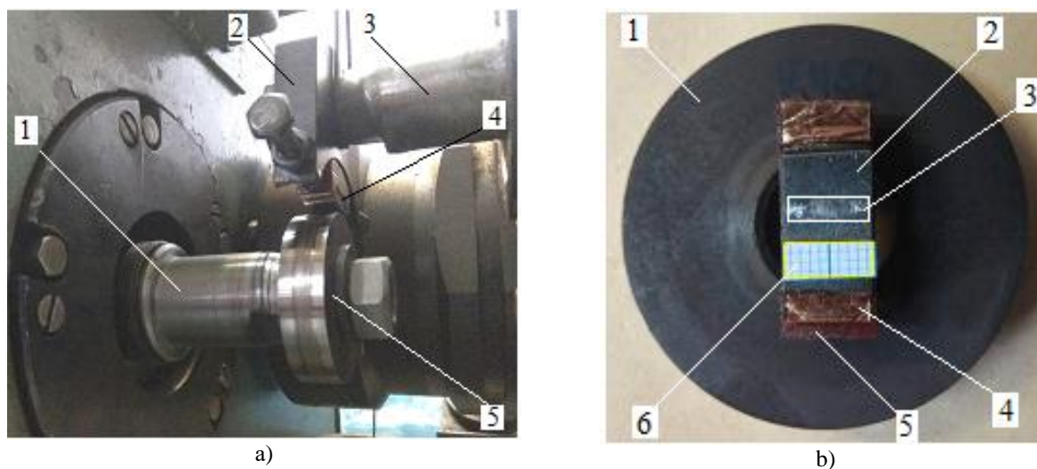
Fig. 3. Methodological support of tribotechnical tests: a - model interface "movable disk - fixed block": 1 - lower shaft; 2 - upper shaft holder; 3 - upper shaft; 4 - sample - block; 5 - sample - disk; b - samples: 1 - disk; 2 - block; 3 - wear mark; 4 - sealant; 5 - shoe holder; 6 - measuring ruler
