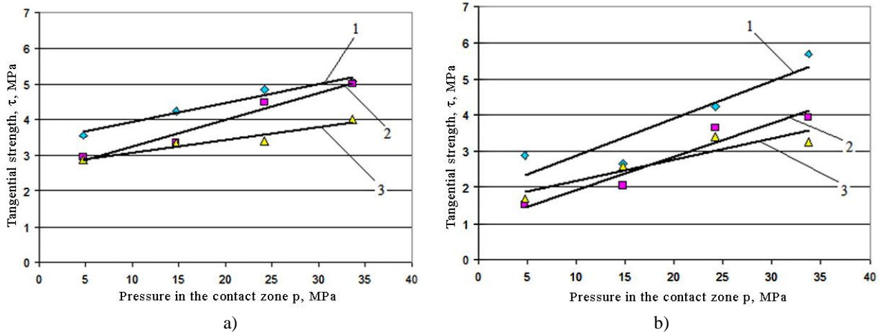
Fig. 7. Tangential strength of adhesive bond in contact of materials "CuCrNiZrTi - 5140H": a - in the environment of TAD-17I transmission oil; b - without lubricant; 1 - mm/s; 2 - mm/s; 3 - shear rate mm/s
