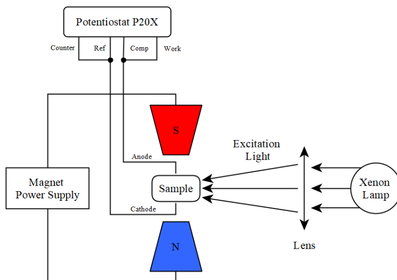
Fig.6. Diagram of the experimental setup for measuring the IVC in an external magnetic field.
