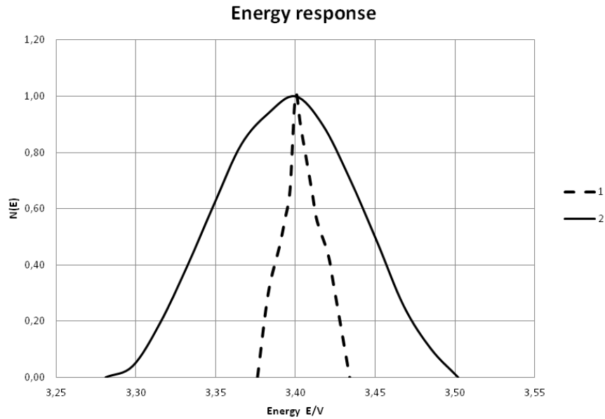
Fig.3. Energy response of the energy analyzer: 1 - for scheme with point source, 2 – for scheme with extended source.
